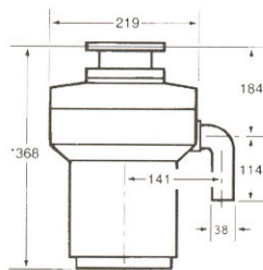
COMMANDER 9000
