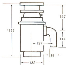
COMMANDER 7000
