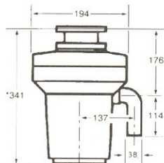
COMMANDER 7500
