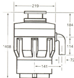
COMMANDER 10000
